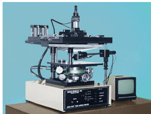
Accu-Coat™ Model 3230-B bench-top screen printer.
