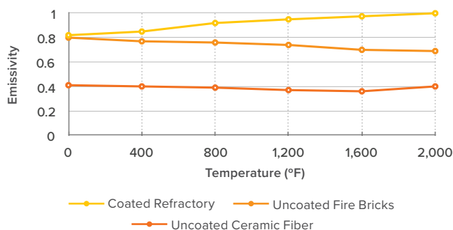
This chart illustrates emissivity of coated versus uncoated firebrick and ceramic fiber.
