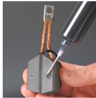
Graphi-Bond™ 551-RN seals sensor in carbon brushes.
