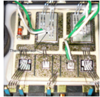
Aremco-Bond™ 556-HT-SP used to bond thermal sensor.
