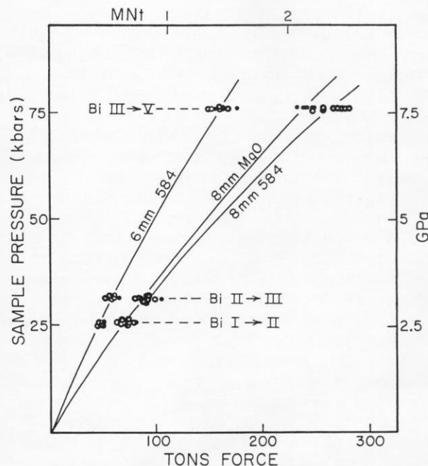
Fig. 3. Bi transition experiments. Clear separation of the forces required to cause transitions to occur is seen as a consequence of change from 6-mm to 8-mm truncated edge length (TEL) on the octahedral facets of the cubic anvils. Open circles are for experiments using Aremc's 584 compound for the pressure medium and gaskets. Filled circles are for experiments using MgO (5% Cr 2 O 3 ) with bonded Al 2 O 3 gaskets. Only for 8 mm Bi III \rightarrow V transitions is there a clear separation of results for the different pressure media. Precision of the pressurization forces required for achieving a transition is typically characterized by a standard deviation \pm 4% of the average pressure. Considering that these results were obtained on a series of experiments in which many parameters such as mix composition, gasket character, and A-C interface pads were also changed, it is possible that still higher precision might be obtained when attention is directed toward uniformity of procedure rather than the effects of variations. Nevertheless, the precision realized here is comparable to that quoted from other laboratories.
