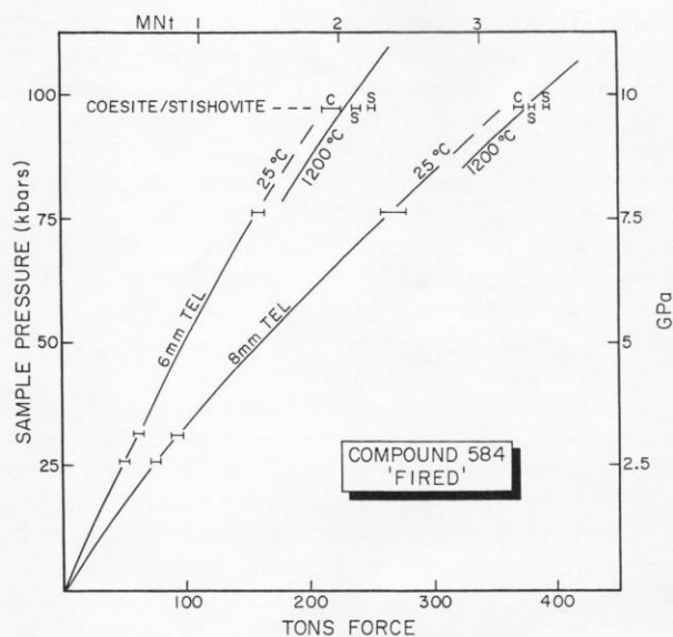
Fig. 4. Performance of Aremc's compound 584 on the Bi transitions at room temperature and for the coesite-stishovite transition at 1200 °C. The error bars on the Bi transitions are 1\sigma bounds on the variations observed in multiple experiments. The error bars (upon individual experiments) for the six C-S experiments reflect the increase in ram pressure experienced during heating of the experiment with a closed hydraulic system. The C or S designation corresponds to the \text{SiO}_2 polymorph recovered at the thermocouple junction even though C may have been recovered at the heater margins.
